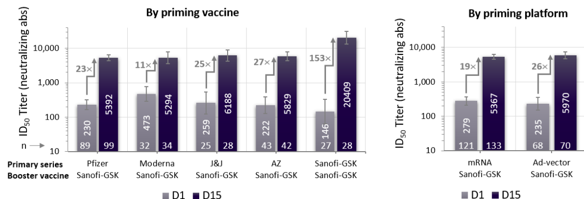
Figure 1b - Pre- vs post-booster neutralizing antibody in ≥56-year old participants. Geometric Mean Titers (GMT) (95% CI).
