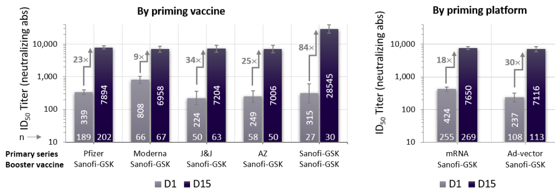
Figure 1a - Pre- vs post-booster neutralizing antibody titers in 18-55-year old participants. Geometric Mean Titers (GMT) (95% CI).
