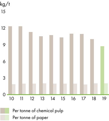
UPM’s COD load per tonne of product
