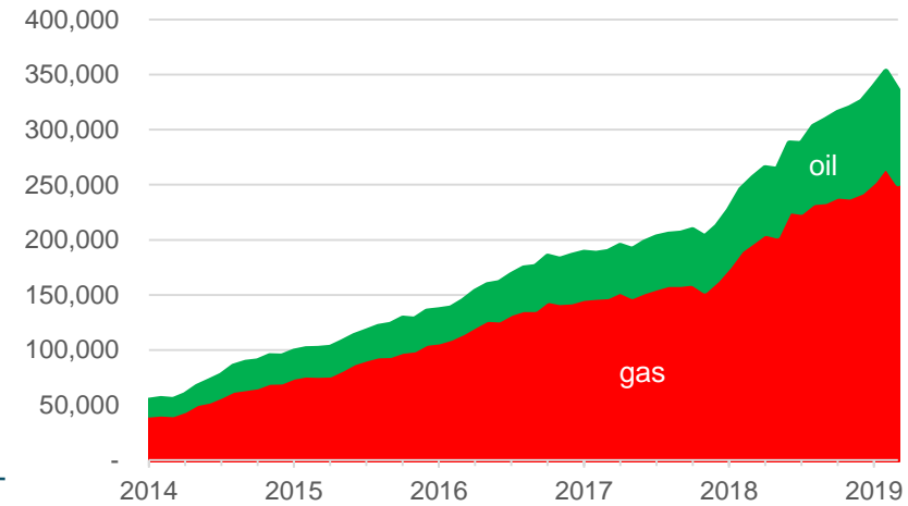
Neuquen shale production (2014-2018) barrels oil equivalent per day
